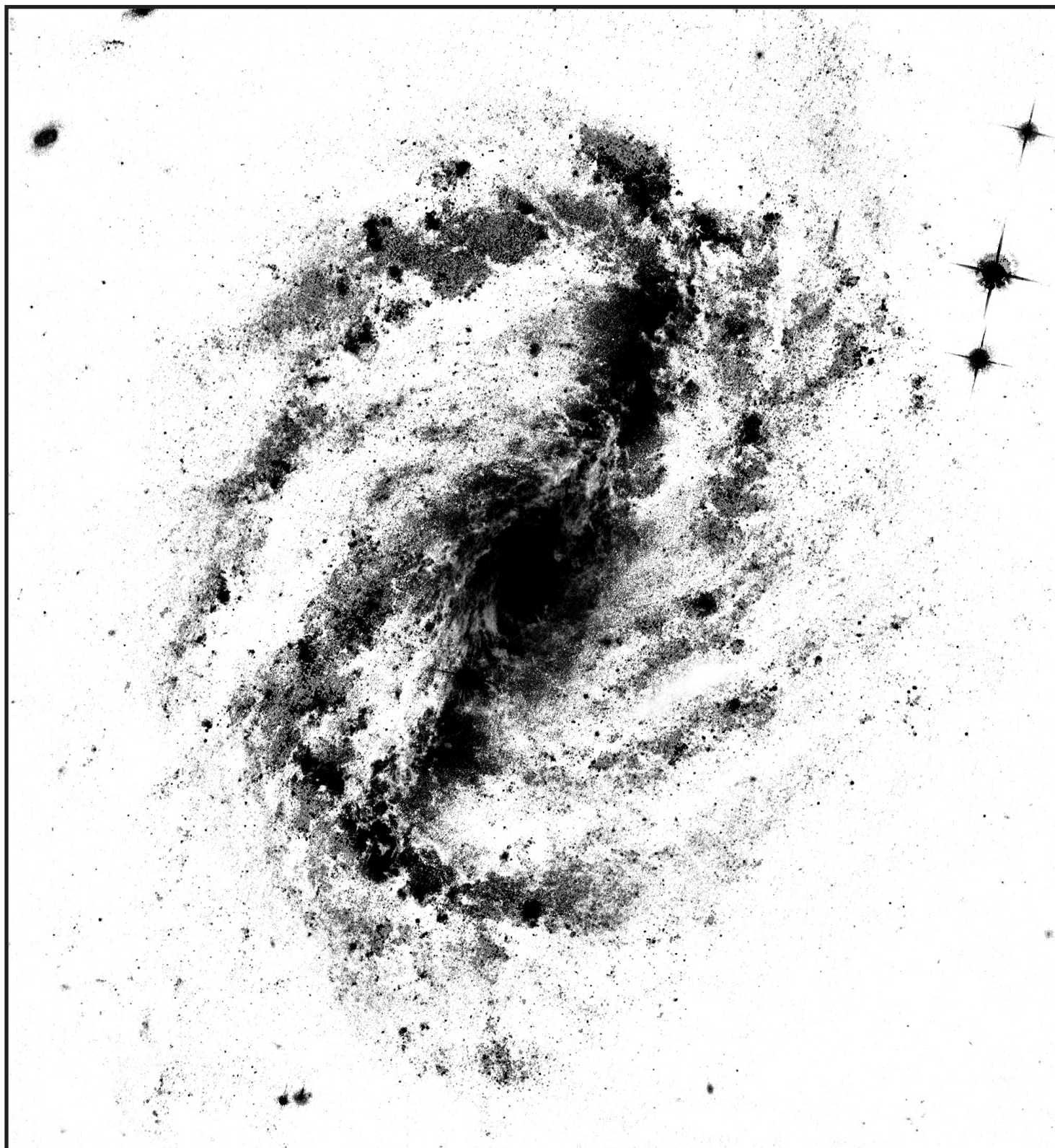
Hubble tactile image: Barred Spiral Galaxy, NGC 6217
