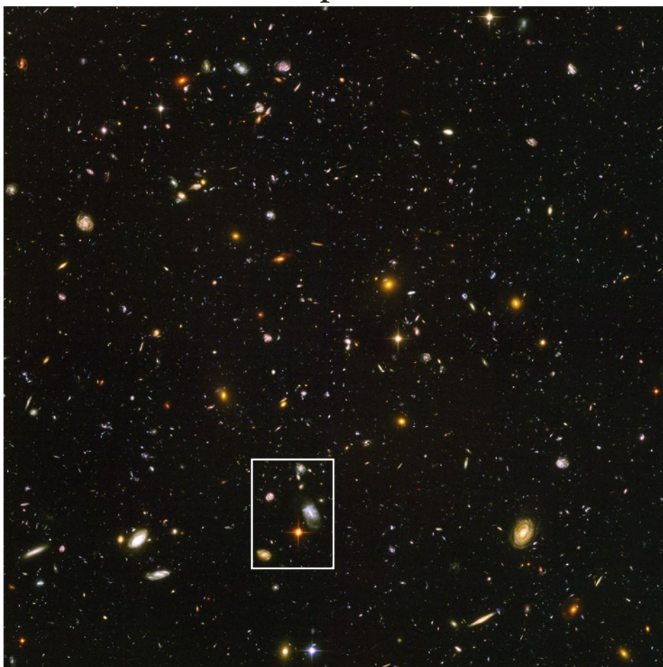
IMAGES: NASA, ESA, S. Beckwith (STScI), and the HUDF Team
